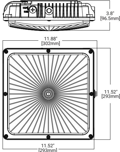
CLCS30S-PC
